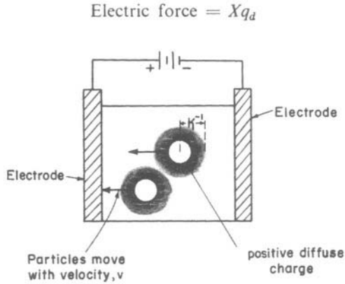
Fig. 6.139. The phenomenon of electrophoresis.
