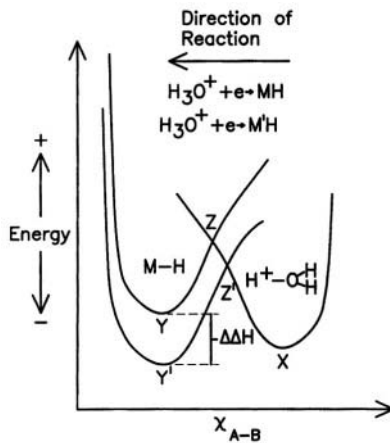
Fig. 9.15. This schematic is subject to the same reservations as that in Figs. 9.9 and 9.10. It shows the potential energy variation during the vibration of M–H and
