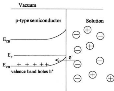
Fig. 7.28. A p -type semiconductor acts as an anode in thermal reaction under dark conditions.
