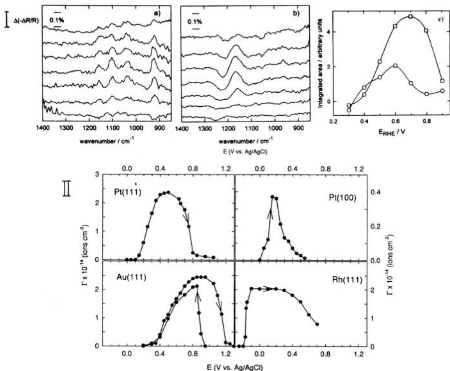
Fig. 6.21. FTIR spectra of Pt(111) in 0.1 M HClO 4 + 1 mM Ti + in (a) the absence and (b) in the presence of 1 mM H 2 SO 4 . (c) Dependence of integrated area on electrode potential for the bands shown in (a) and (b). (O) perchlorate bands, and (□) bisulfate bands. (Reprinted with permission from N. S. Marinković, W. R. Fawcett, J. X. Wang, and R. R. Adžić, J. Phys. Chem. 99 :17490, Figs. 3 and 4, copyright 1995, American Chemical Society.) (II) Bisulfate coverages in 0.1 M HClO 4 supporting electrolyte, as measured by a radiotracer technique on: Pt(111), c_{\text{H}_2\text{SO}_4} = 1 \text{ mM} ; Pt(100), c_{\text{H}_2\text{SO}_4} = 0.1 \text{ mM} ; Au(111), c_{\text{H}_2\text{SO}_4} = 0.5 \text{ mM} ; and Rh(111), c_{\text{H}_2\text{SO}_4} = 1 \text{ mM} . (Reprinted from P. A. Rikvold, M. Gamboa-Aldeco, J. Zhang, M. Han, Q. Wang, H. L. Richards, and A. Wieckowski, Surf. Sci. 335 :389, copyright 1995, Fig. 6; M. Gamboa-Aldeco et al., J. Electroanal. Chem. 348 :451, copyright 1993, Figs. 2 and 3; and Z. Shi et al., J. Electroanal. Chem. 366 :317, copyright 1994, Fig. 5, with permission from Elsevier Science.)
