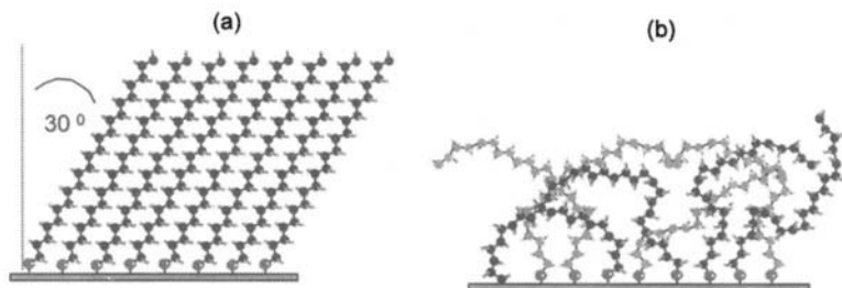
Fig. 6.113. Models for (a) 6-mercaptohexadecanol and (b) 22-mercapto-dodecanoic acid, adsorbed on gold substrates investigated by near-edge X-ray absorption fine structure (NEXAFS) spectroscopy and X-ray photoelectron spectroscopy. (Reprinted from O. Dannenberger, K. Weiss, H. J. Himmel, B. Jäger, M. Buck, and Ch. Wöll, Thin Solid Films 307 : 183, copyright 1997, Fig. 6, with permission from Elsevier Science.)
