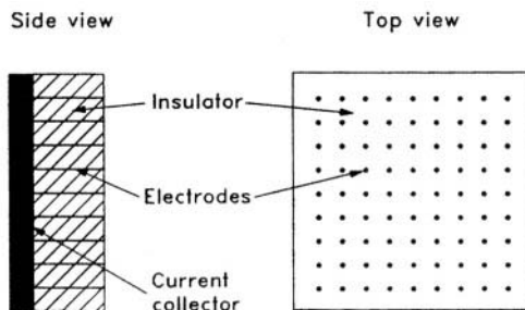
Fig. 7.34. An ensemble of ultramicroelectrodes. (Reprinted from E. Gileadi, Electrode Kinetics for Chemists, Chemical Engineers, and Materials Scientists , VCH Publishers, 1993, p. 450. Copyright © 1993 John Wiley. Reprinted by permission of John Wiley & Sons, Inc.)
