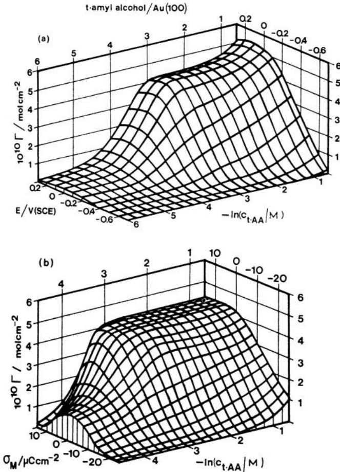
Fig. 6.58. Three-dimensional graphs representing the surface excess (approximately equivalent to the number of adsorbed molecules) of ter -amyl alcohol calculated with respect to (a) the electrode potential and (b) the charge density. The electrical variable varies along the axis "normal" to the plane of the figure. The maximum surface excess corresponding to the plateau on both graphs is equal to 4.4 \times 10^{-10} \text{ mol cm}^{-2} . In this figure \sigma_M = q_M . (Reprinted from J. Richer and J. Lipkowski, J. Electroanal. Chem. 251 :217, copyright 1988, Fig. 12, with permission of Elsevier Science.)
