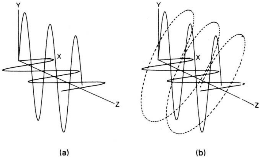
Fig. 7.57. Perspective view of the x and y components of an elliptically polarized wave. The ellipse results as a resultant of the two components. (Reprinted from R. A. Serway, C. J. Moses, and C. A. Moyer, Modern Physics , Saunders College Publishing, 1997, p. 208.)
