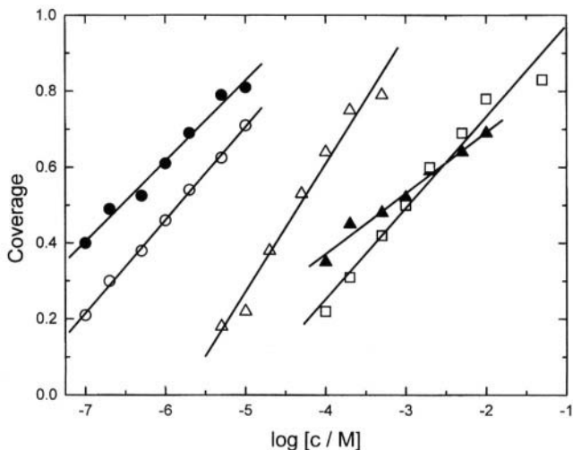
Fig. 6.117. Adsorption isotherms for various organic species on platinum in 0.01 N HCl solution, obtained with the radiotracer technique: valeriac acid (▲), butanol (□), benzoic acid (△), naphthoic acid (●), naphthol (○). All the data are taken at the maximum adsorption potential. (Reprinted from J. Jeng, dissertation, Texas A&M University, 1991.)
